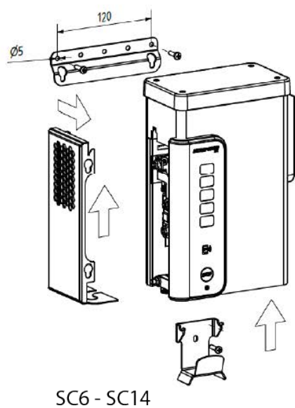
Fig. 2 Installation
