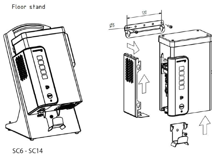
Fig. 5 Installation options
